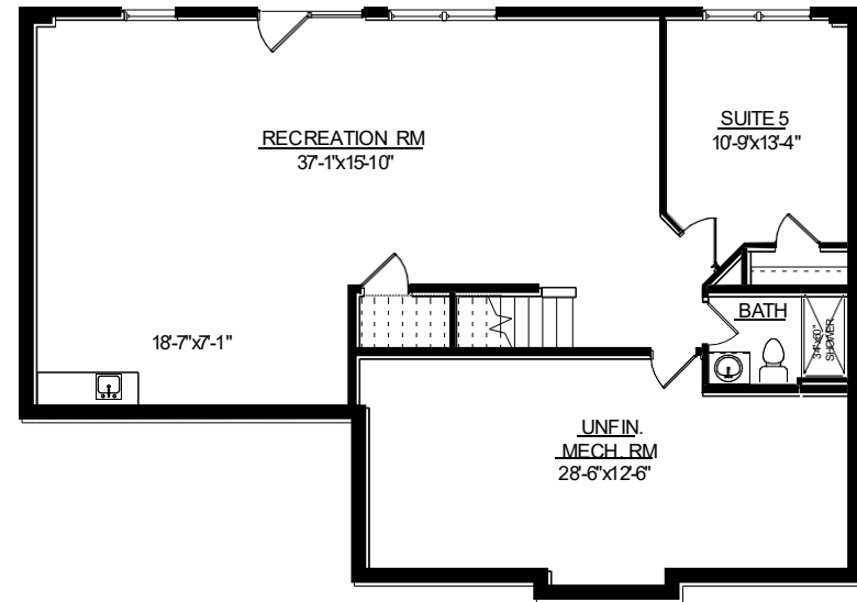
OPT. BASEMENT PLAN
