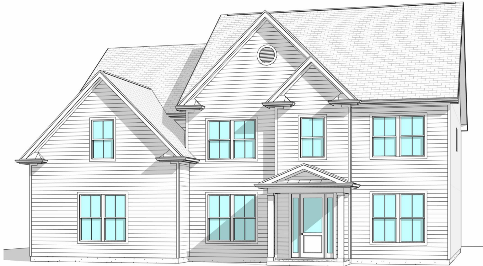
Elevation - A (Side Load)
