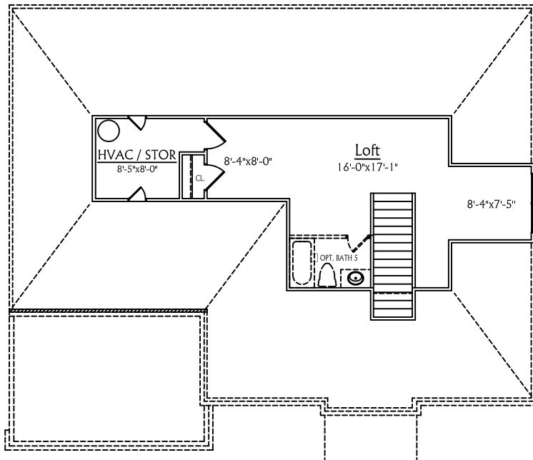
THIRD FLOOR PLAN - ELEV. 'C'
