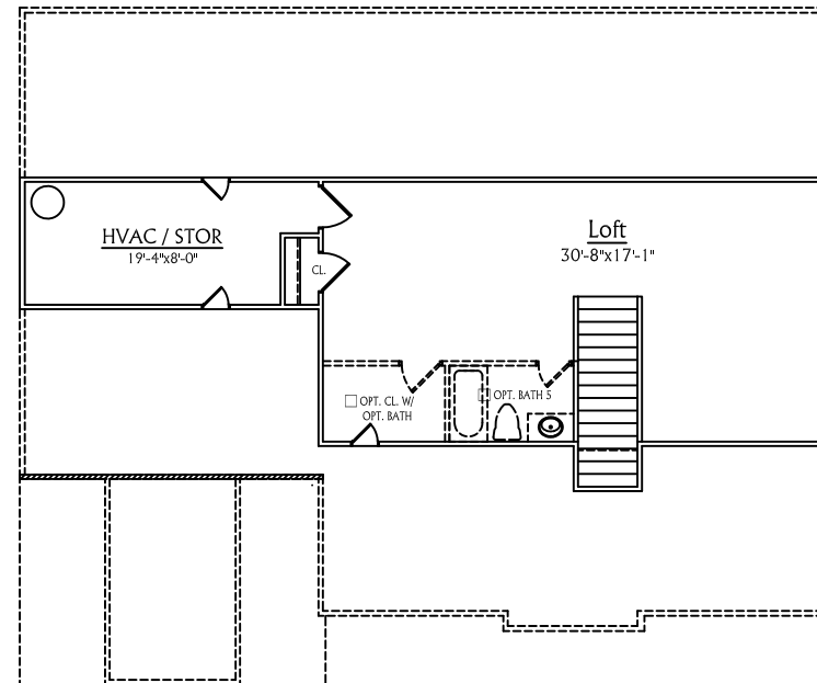
THIRD FLOOR PLAN - ELEV. 'A & B'
